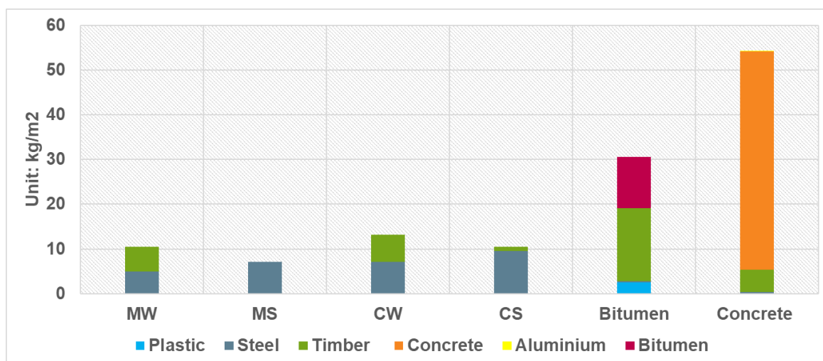
Figure 6: Mass composition per m² of the roof designs
