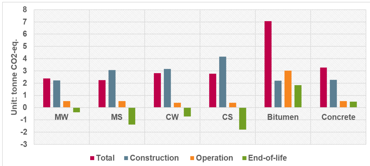
Figure 9: GWP per each life cycle stage
