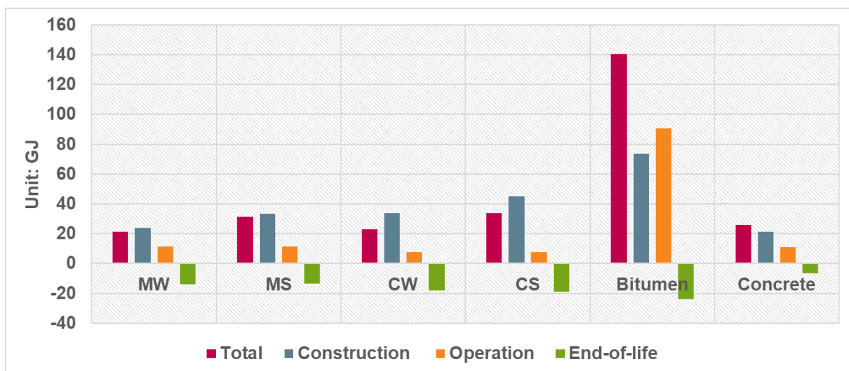
Figure 13: PED per each life cycle stage
