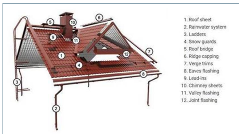
Figure 1: Roof structure
